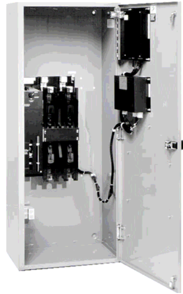
CTS SERIES ATS 400 amp, 2 pole
